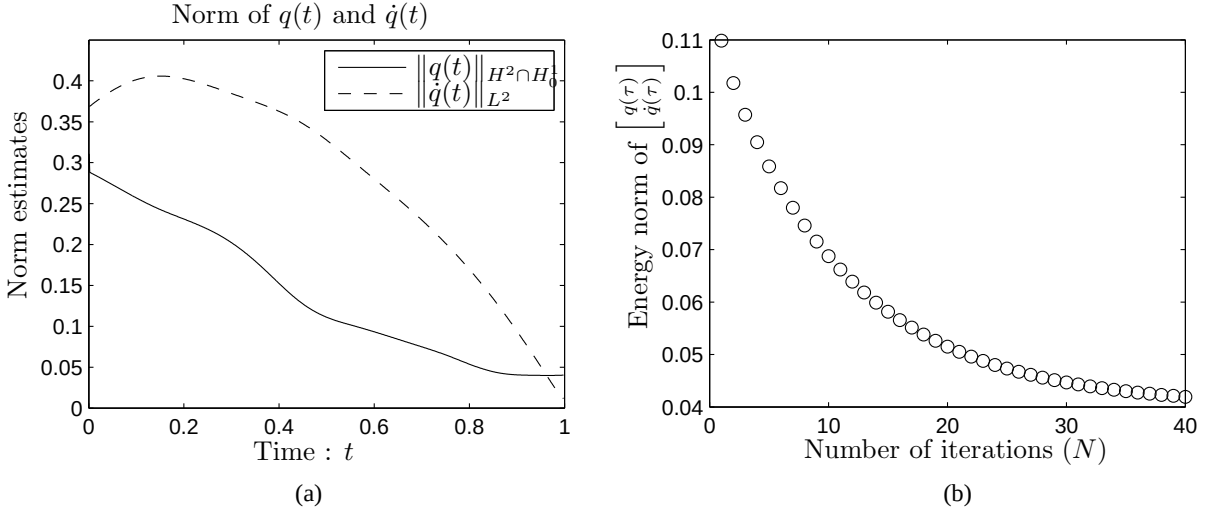
Figure 4.3: (a) The norm of the solution of the controlled beam equation, with u = u_h and the initial state q_0(x) = x^5(1-x)^5 , q_1(x) = -q_0(x) . (b) The energy of the solution of the controlled beam at time \tau versus the number of terms N in the approximation of u_h .
