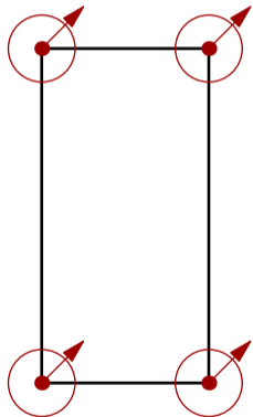
Bogner-Fox-Schmit (BFS)
