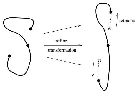
FIG. 2.1. ( inspired from the book [10, page 2058] ) – When a macroscopic deformation is applied, a polymer chain is transformed into a new conformation. The new chain is on the curve which is the affine transformation of the initial curve. The new position of each segment is obtained by retraction, preserving the initial lengths.
