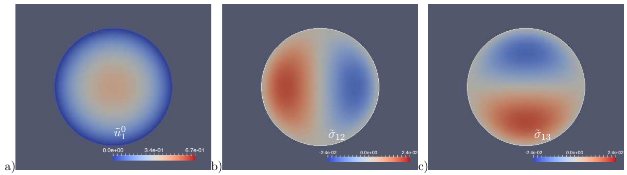
Figure 8: Geometry (I): normalized fields at x_1 = 0.25 : a) velocity profile \tilde{u}_1^0 , b) extra-stress \tilde{\sigma}_{12} , c) extra-stress \tilde{\sigma}_{13} .
