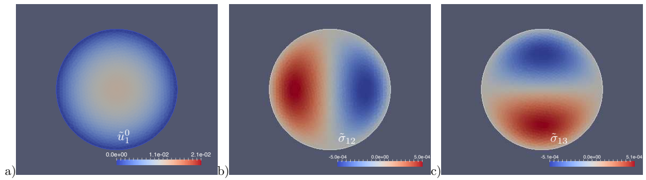
Figure 10: Geometry (II): normalized fields at x_1 = 0.125 : a) velocity profile \tilde{u}_1^0 , b) extra-stress \tilde{\sigma}_{12} , c) extra-stress \tilde{\sigma}_{13} .
