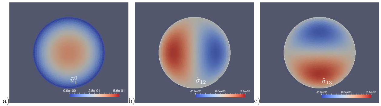
Figure 17: Geometry (IV): normalized fields at x_1 = 0.25 : a) velocity profile \tilde{u}_1^0 , b) extra-stress \tilde{\sigma}_{12} , c) extra-stress \tilde{\sigma}_{13} .
